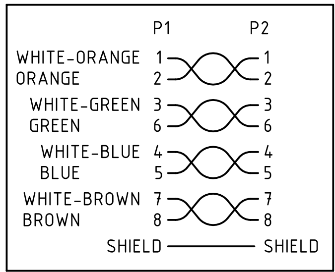
circuit diagram
