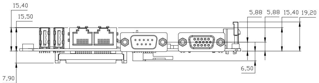
Figure 2.5 Board Dimension layout (Coastline)
